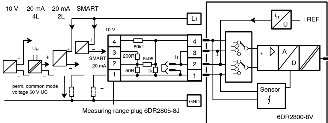
Block diagram mV-module 6DR2800-8V
