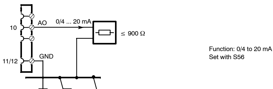
Figure 4-14 Connection AO
