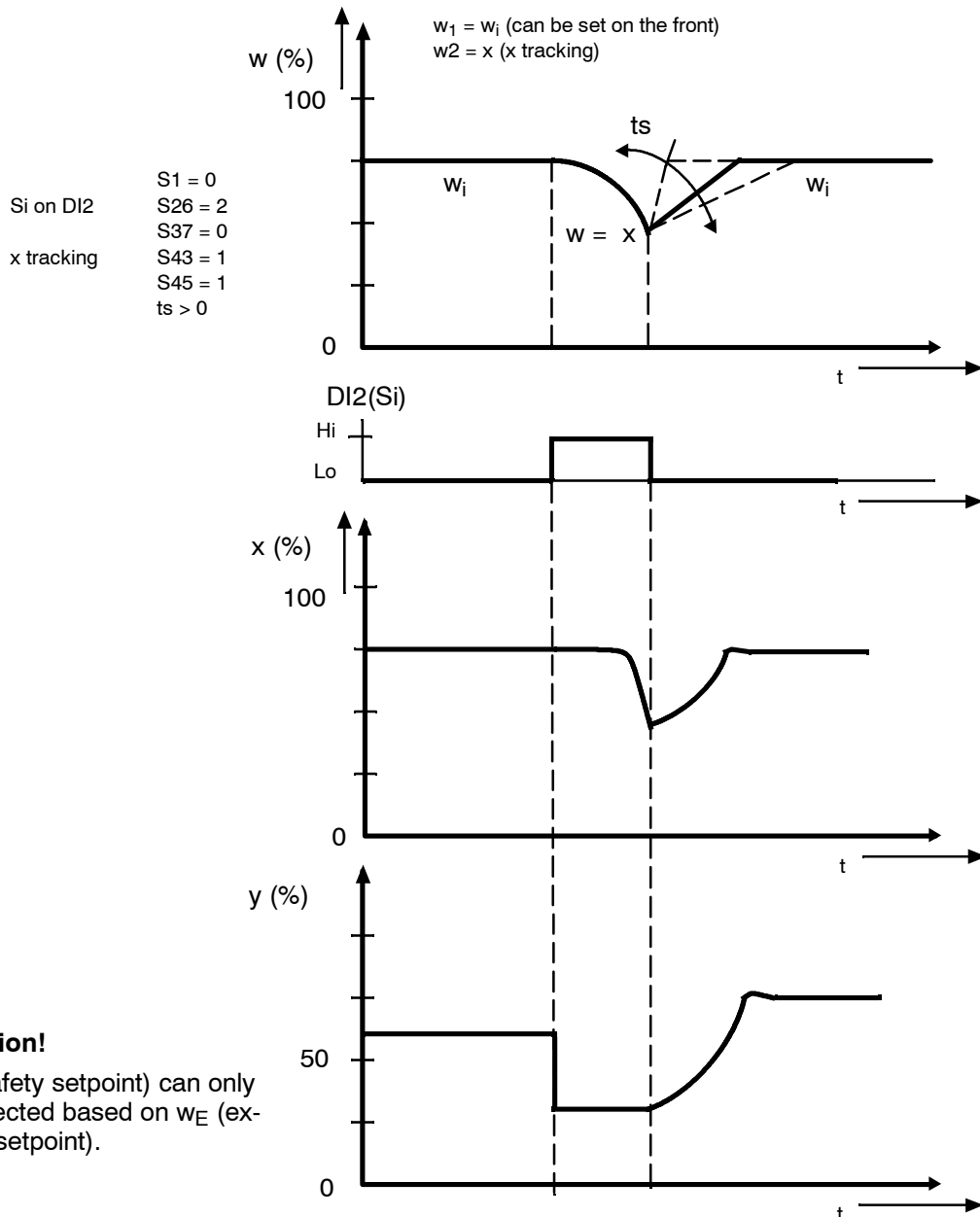
Figure 7-4 Setpoint curve according to example 4
