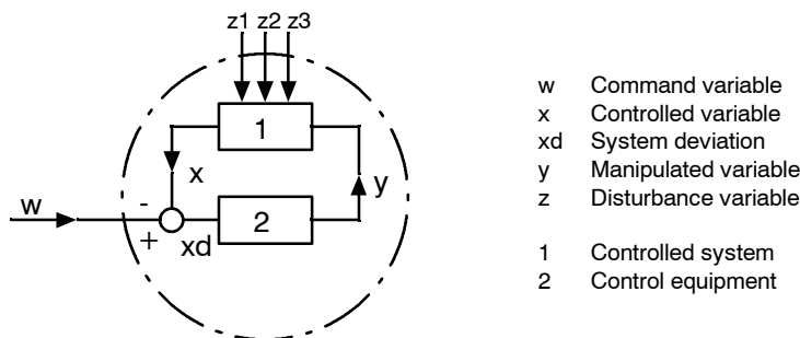
Figure 1-1 Function diagram of control loop
