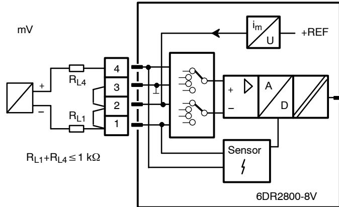
Block diagram mV-module 6DR2800-8V
