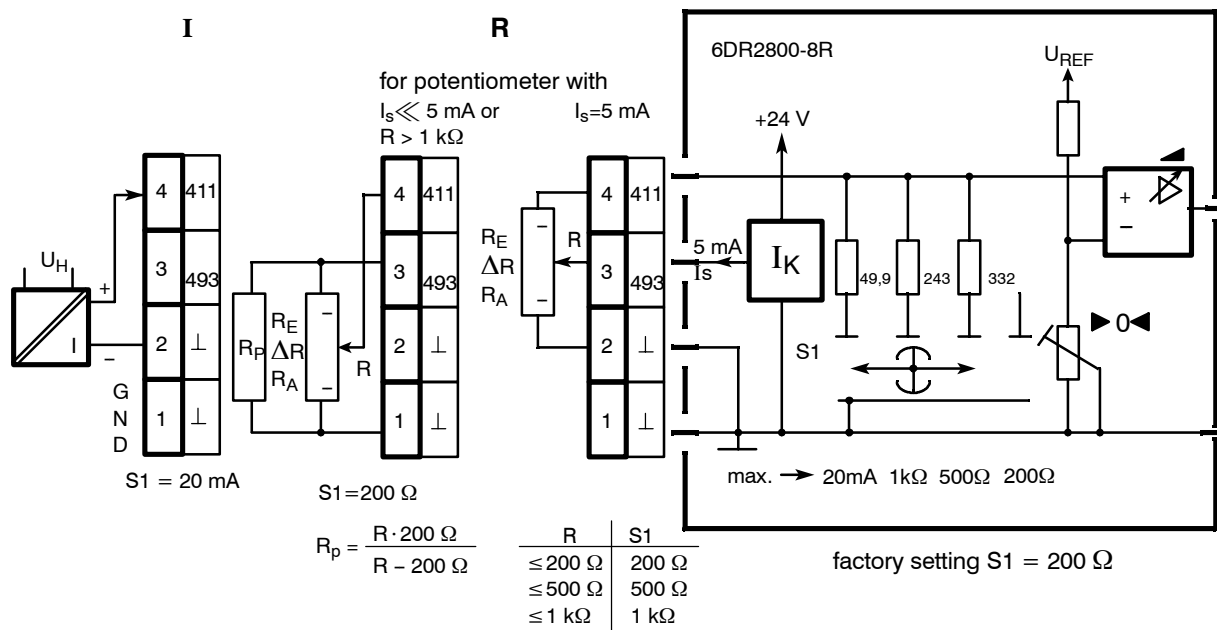
Figure 4-18 Connection R-module 6DR2800-8R
