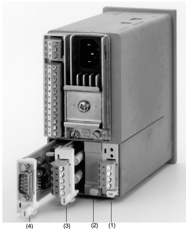
Figure 4-7 Rear of controller
