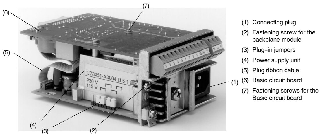
Figure 8-3 Backplane module
