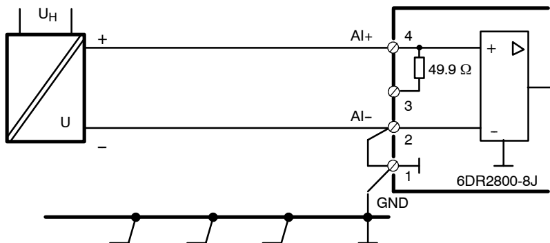
Figure 4-30 Connection of a floating voltage supply
